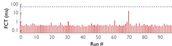
Figure 2: FCT of the short flow across 100 attempts of replay with socket calls. The blue dashed-line is 49 ms.
